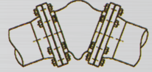
Angular Deflection
